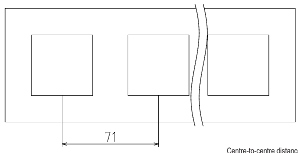
Centre-to-centre distance
