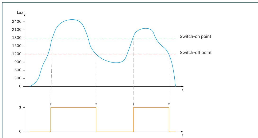
Figure 9: Diagram – Threshold Switch / Hysteresis
