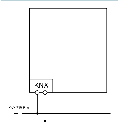
Figure 1: Wiring diagram
