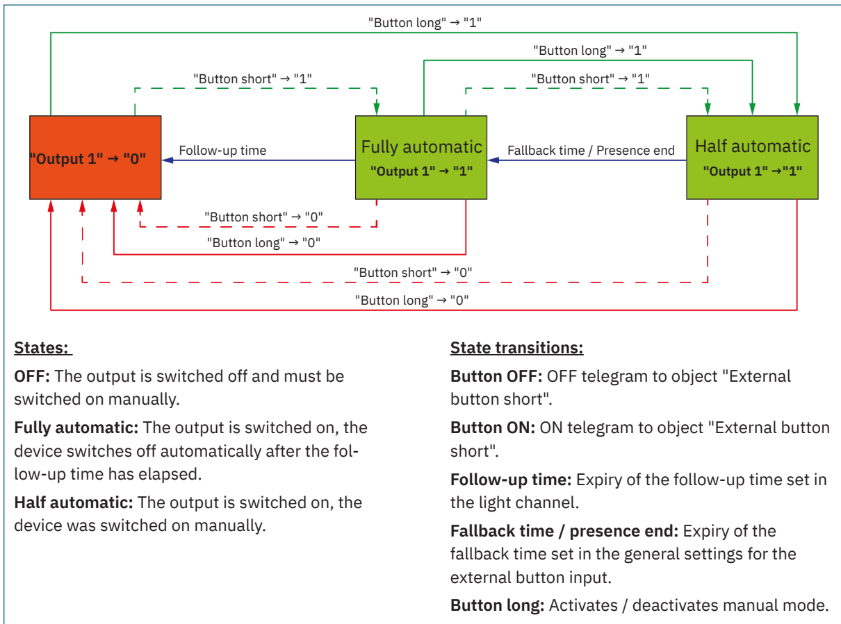
Figure 7: Process diagram – Half automatic without orientation light
