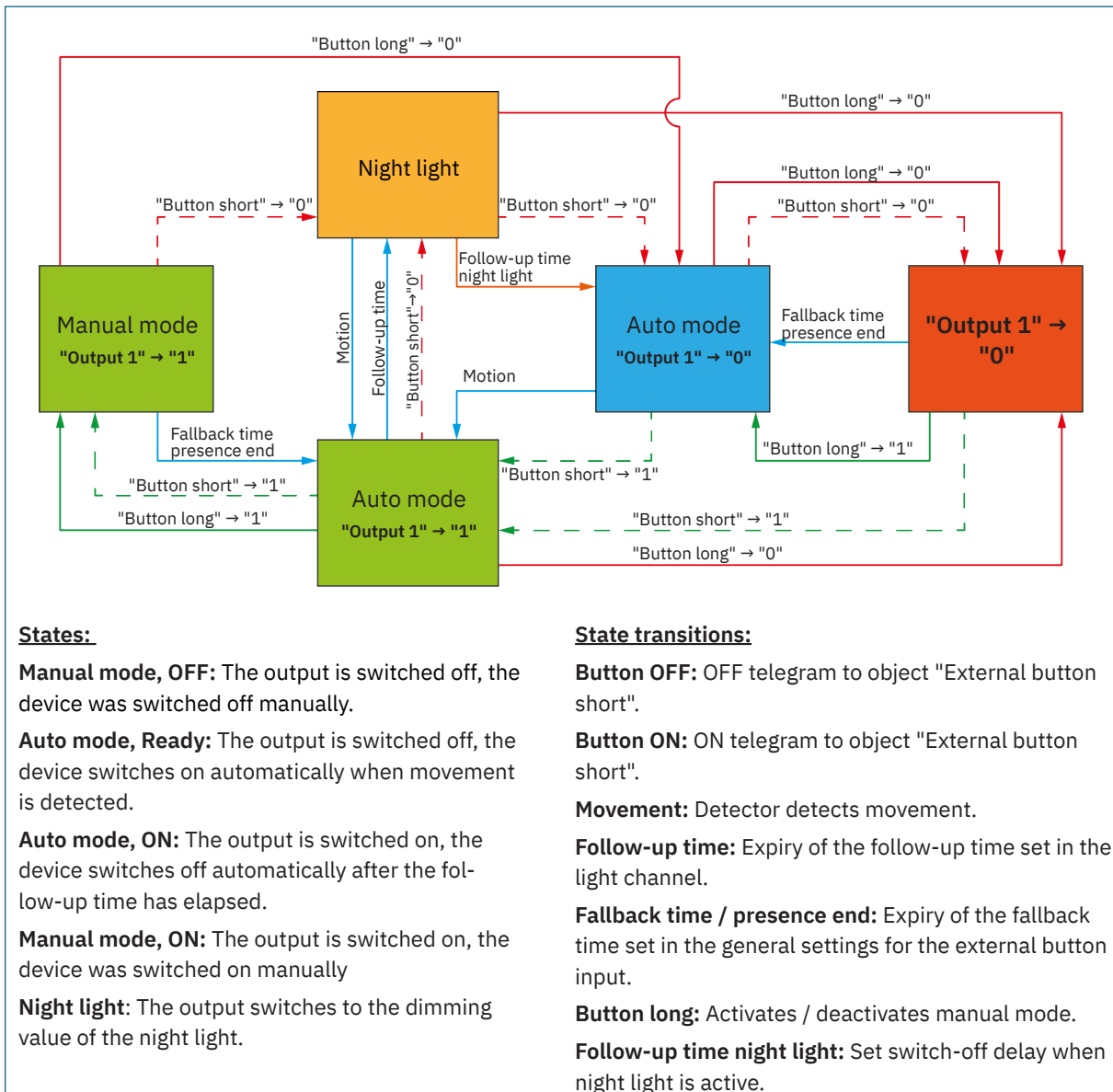
Figure 6: Process diagram – Fully automatic with orientation light
