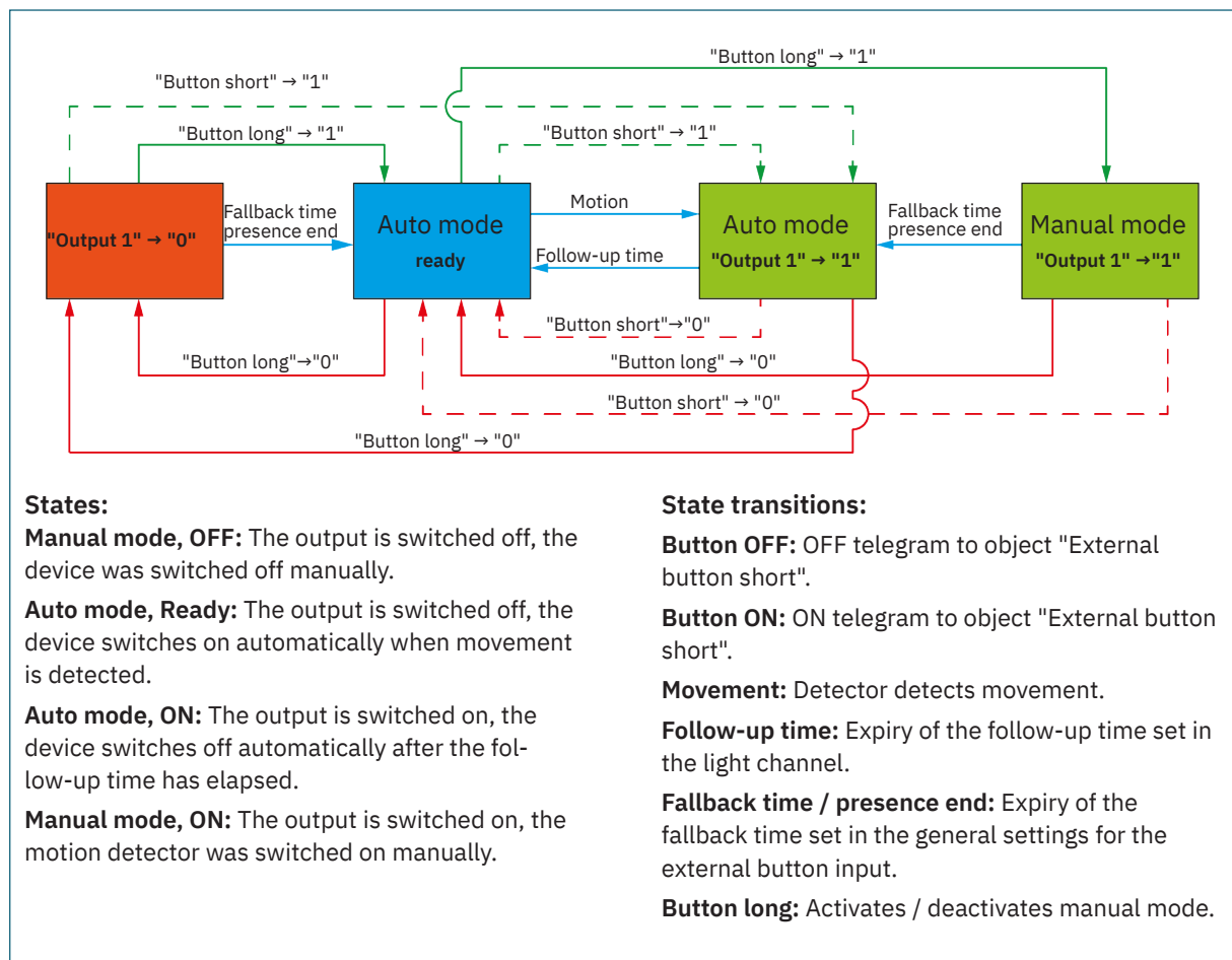
Figure 5: Process diagram – Fully automatic without orientation light
