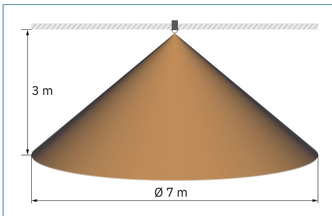
Figure 3: Detection area
